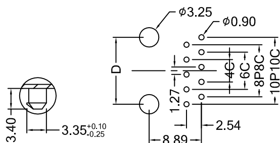
Detail Z
